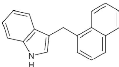
3-(Naphthalen-1-yl-Methyl)-1 H -Indol
