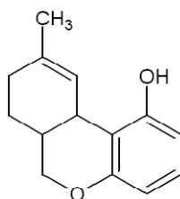
9-Methyl-tetrahydro-6 H -Benzo[c]chromen-1-ol
