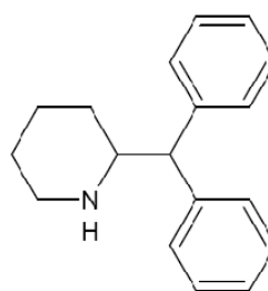
2-(Diphenylmethyl)-Piperidin
