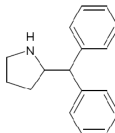
2-(Diphenylmethyl)Pyrrolidin
