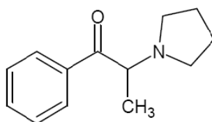
1-Phenyl-2-(Pyrrolidin-1-yl)-Propan-1-on
