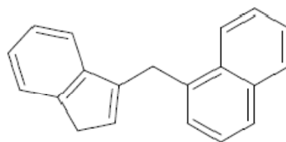
1-(1 H -Inden-3-yl-Methyl)-Naphthalen
