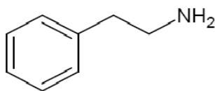
2-Phenylethanamin
